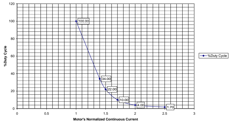
%Duty Cycle vs Motor's Normalized Continuous Current (%Duty Cycle = Time "on"/("Time"on" + Time"off") Motor Attached to 12"x12"x1/2" Aluminum Heat Sink, Maximum Winding Temp = 130°C, Ambient = 25°C
