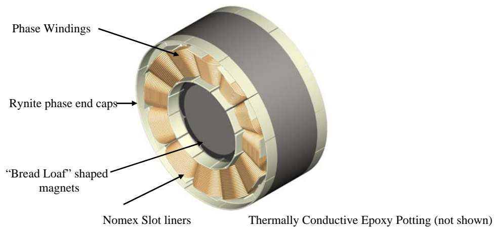
Figure 5: Insulation System. UL Class 180 H
