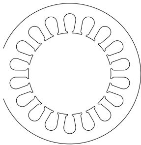
Figure 3: Minimized, non-overlapping end turns
