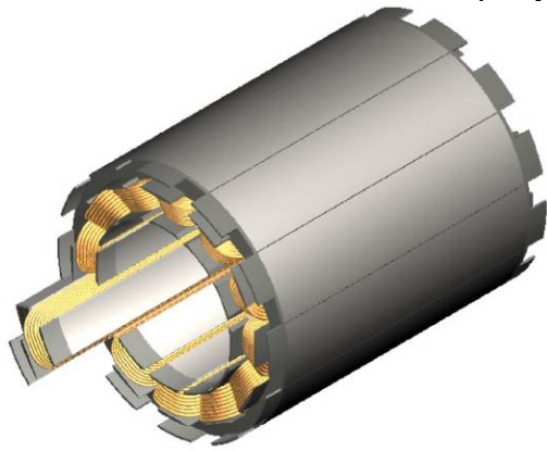
Figure 1. T-LAM™ Stator Prior to epoxy encapsulation
