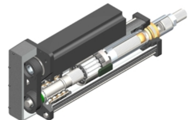
I Series actuators (above) and FT Series actuators (right) offer Exlar's roller screw technology with motor type and mounting flexibility.
