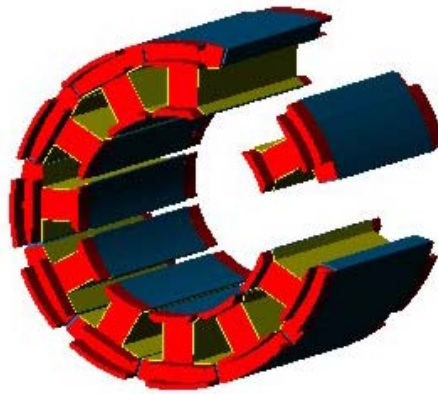
Figure 4 – T-LAM Core Structure
