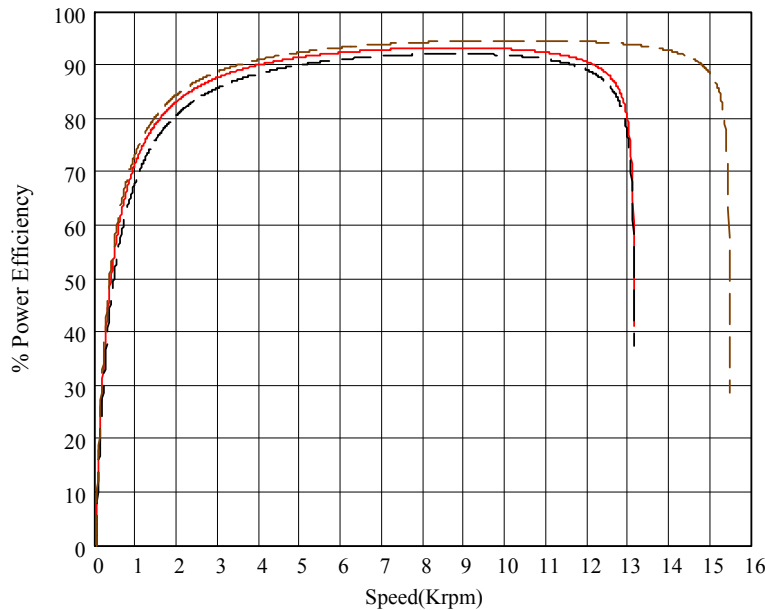
SLM90-238, Different Winding Temperature, 25°C Ambient Dash Brown = T-Lam - 40% less R, 50% less Rth, 100°C Winding Solid Red = T-Lam - 40% less R, 130°C Winding Dash Black = Original Solid Core, 130°C Winding
