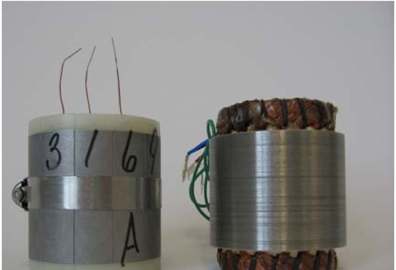
T-LAM Stator
