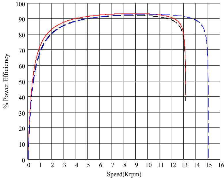
Figure 14 – SLM90-238 Continuous Power Efficiency Curve
