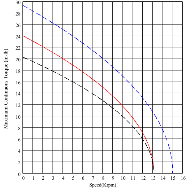
Figure 12 – SLM90-238 Continuous Torque-Speed Curve
