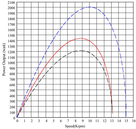
Figure 13 – SLM90-238 Continuous Power-Speed Curve
