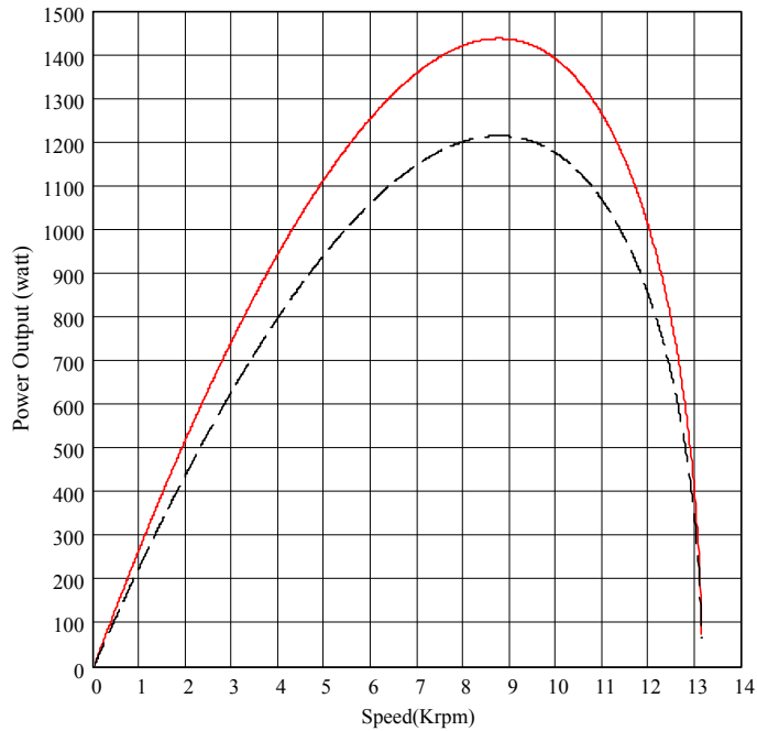
Figure 8 – SLM90-238 Continuous Power-Speed Curve
