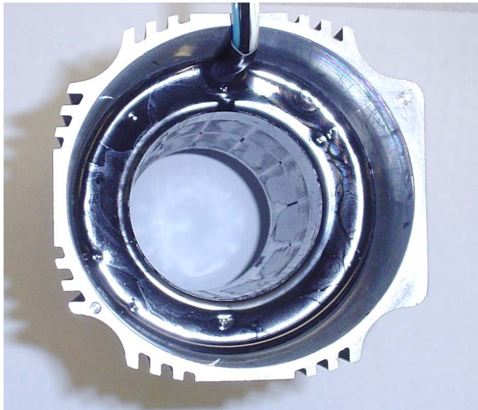
Figure 10 – T-LAM Stator Potted with Thermally Conductive Epoxy
