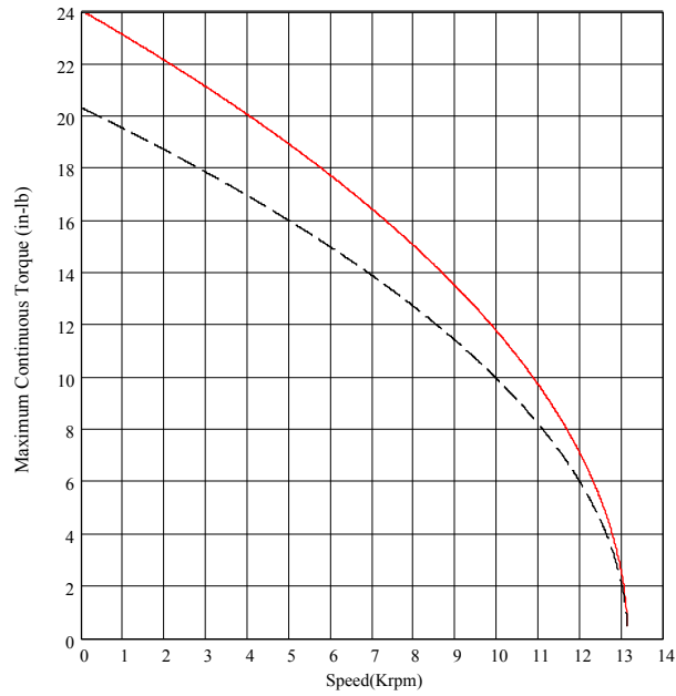
Figure 7 – SLM90-238 Continuous Torque-Speed Curve
